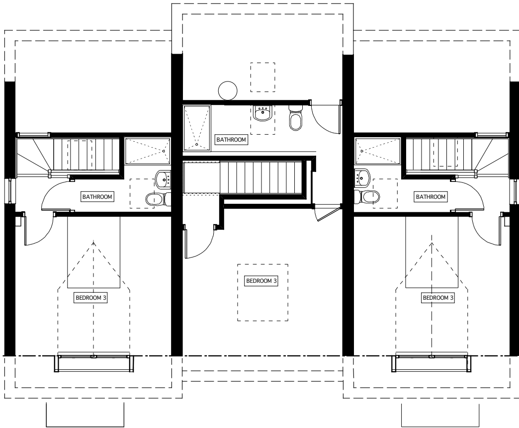
SECOND FLOOR PLAN 134/136/138 HIGH ROAD, TRIMLEY ST. MARY scale 1/100
